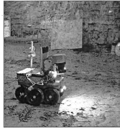
Fig. 3. The Kurt3D robot scanning underground.
